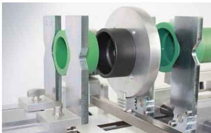
Add-on movable clamps
